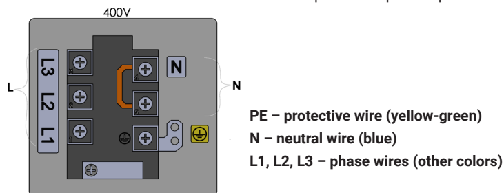
Figure 20. connecting the unit to the mains
