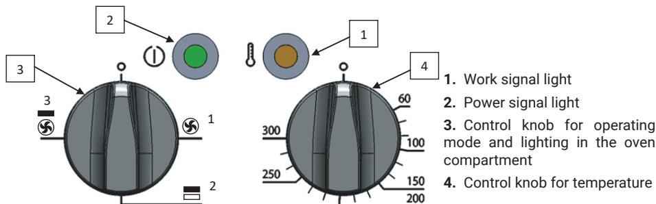
Figure 14. ECO Oven Controls
