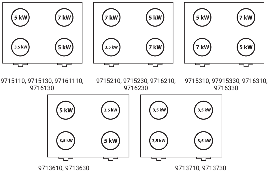
Figure 4. Burner location in the four-burner stove (schematic)
