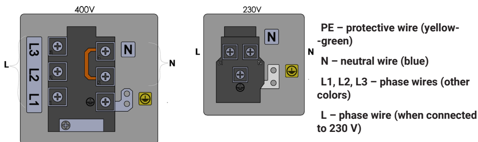
Figure 21. Connecting the unit to the mains for ECO kitchen in accordance according to the label on the appliance.
