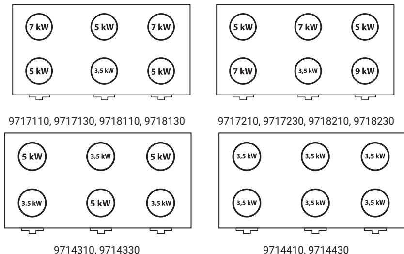
Figure 5. Burner location in the six-burner stove (schematic)
